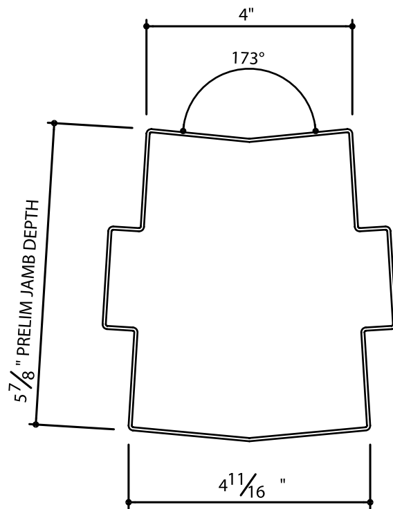
SEGMENTED MULLION DETAIL
