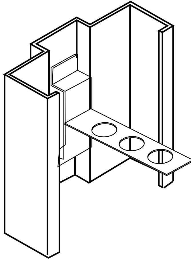
Yoke and Strap Anchor
