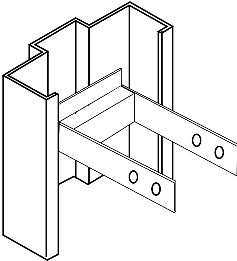
Steel Stud Wood Strap Combo
